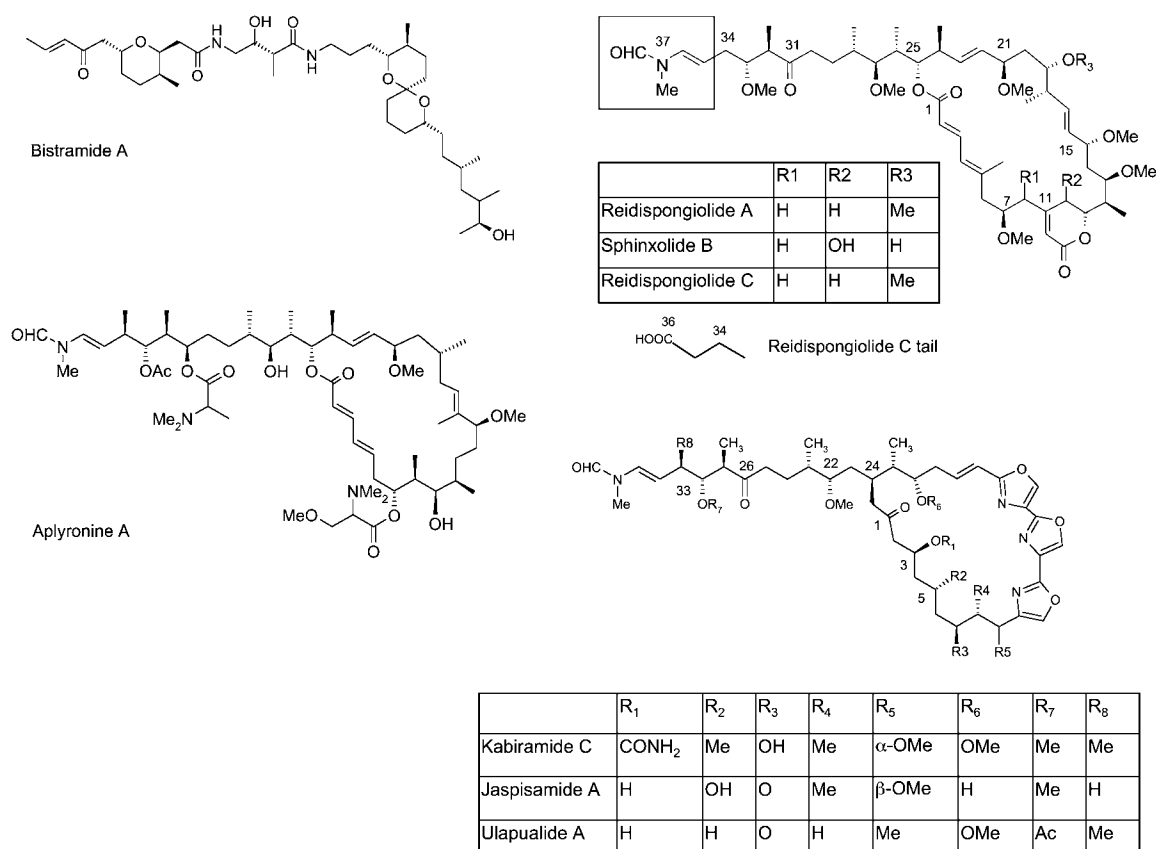
FIGURE 1 Molecular structures of macrolides bistramide A, reidspongiolide A, sphinxolide B, reidspongiolide C (the macrolide tail of reidspongiolide C differs from that of reidspongiolide A and sphinxolide B in the boxed region), kabiramide C, jaspisamide A, ulapualide A (which share a trisoxazole macrolide ring), and aplyronine A that bind to the gelsolin binding site on actin.
